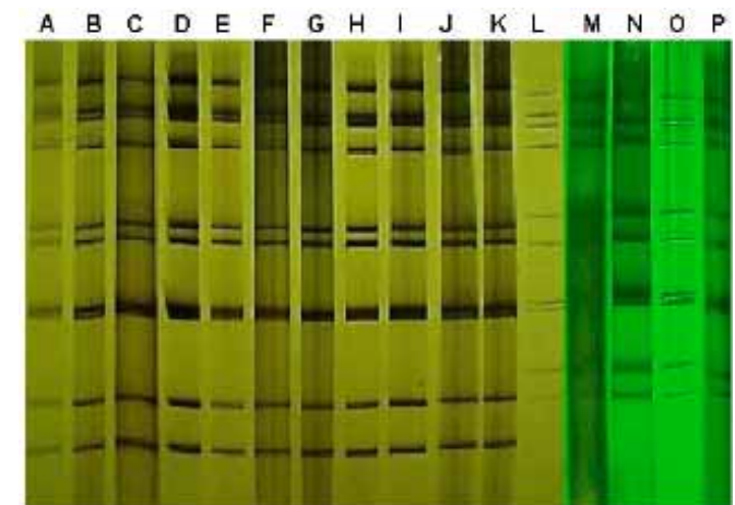
Fig. (2). PAGE of rotaviruses showing the same long electropherotype L6 found in specimens from 2003 (A), 2004 (B-C), 2005 (D-J) and 2006 (K), and the distinct short patterns S3 (L), S2 (M-N), S4 (O) and S1 (P) obtained in 2006.
