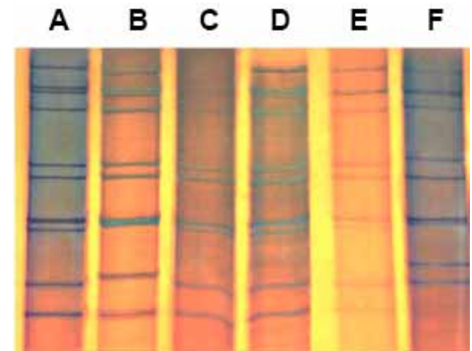
Fig. (1). PAGE of group A rotavirus 10 dsRNA genome with the typical tight triplet formed by segments 7, 8 and 9. Electropherotypes: L1 (A), L4 (B), L9 (C), L10 (D), L8 (E), and S1 (F).
